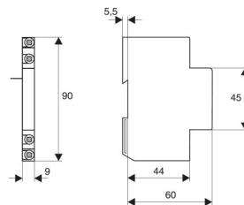
Auxiliary contact
